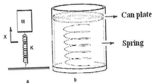
Fig. 1. a) The proposed model for predicting of height changes of can plate during feeding process of sliver from can. b) Can structure
